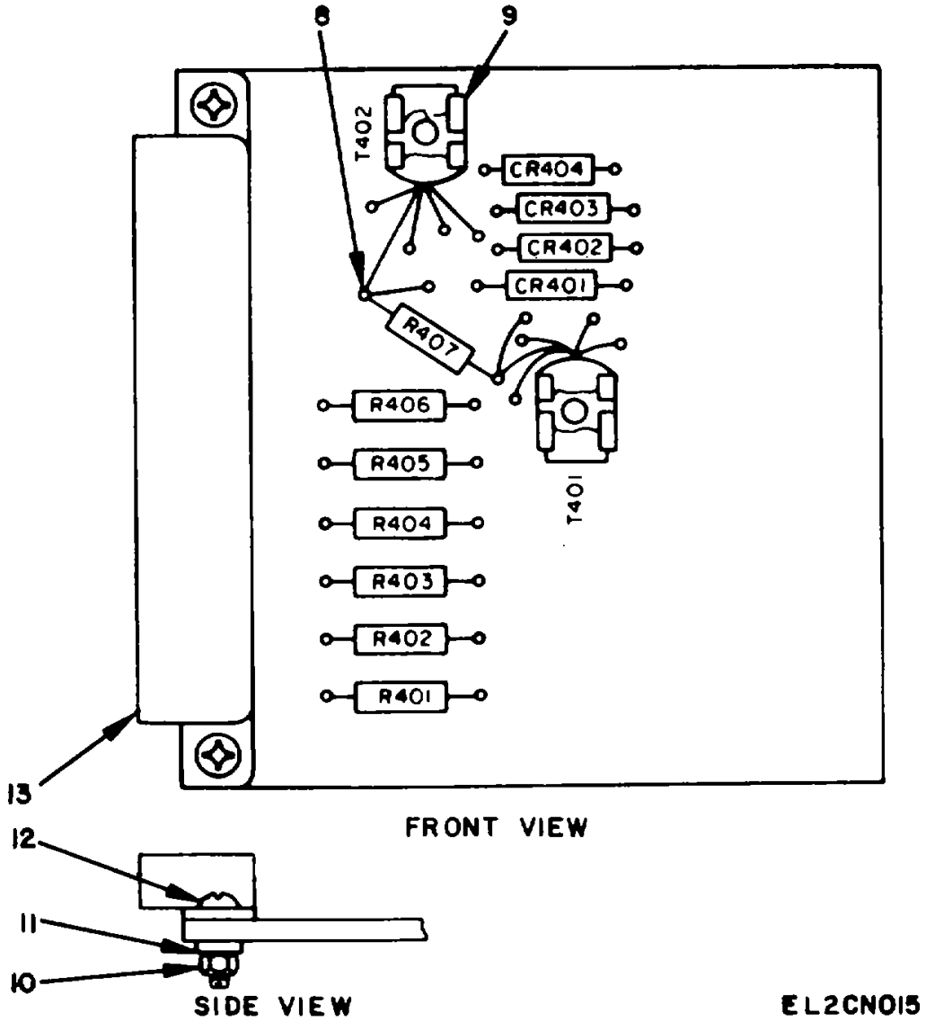
Figure 13. Component Assembly, Card A02V3068-1.
