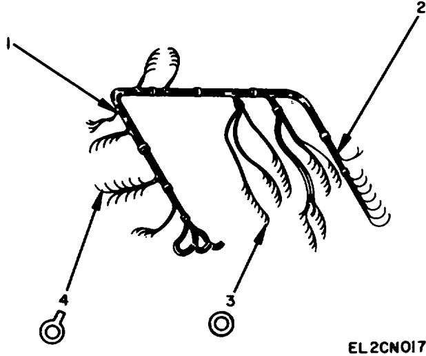
Figure 15. Cable Harness 114E5987-5.
