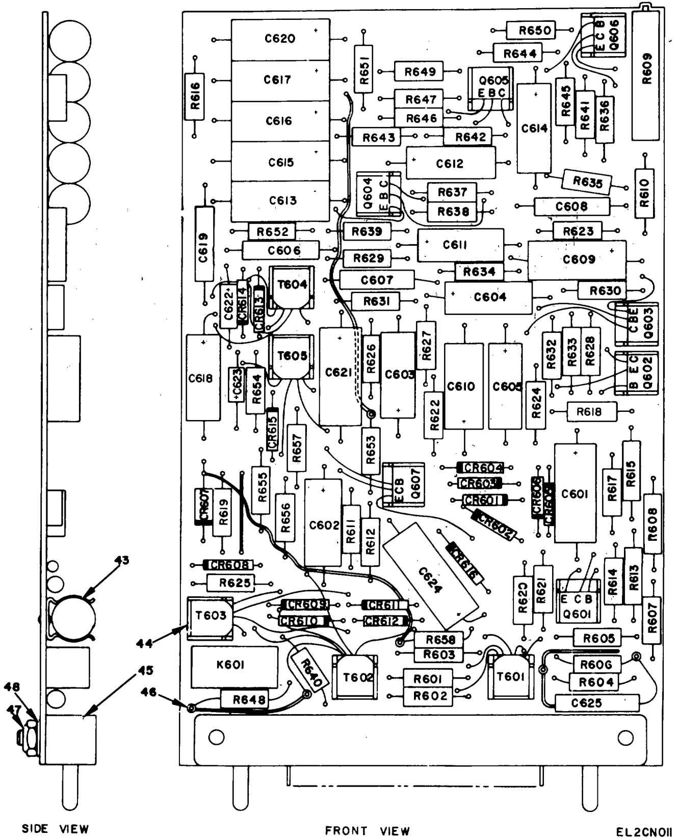
Figure 10. Component Assembly, Actuator Simulator Card A02V3048-2 (Sheet 1 of 2).
