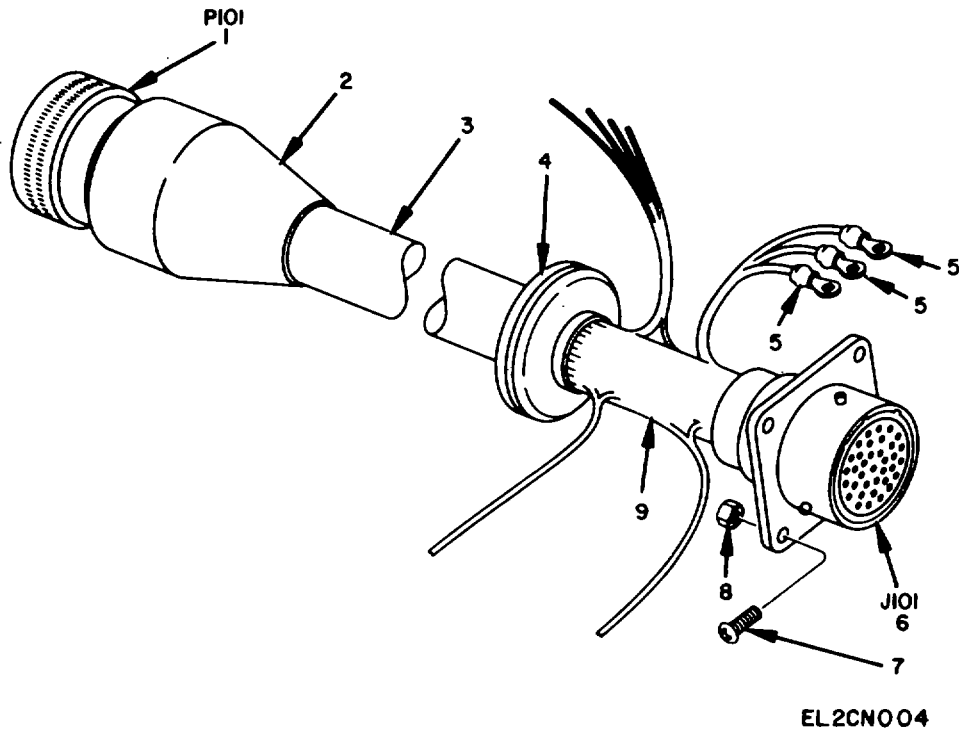
Figure 4. Cable Assembly 114V3062-1.
