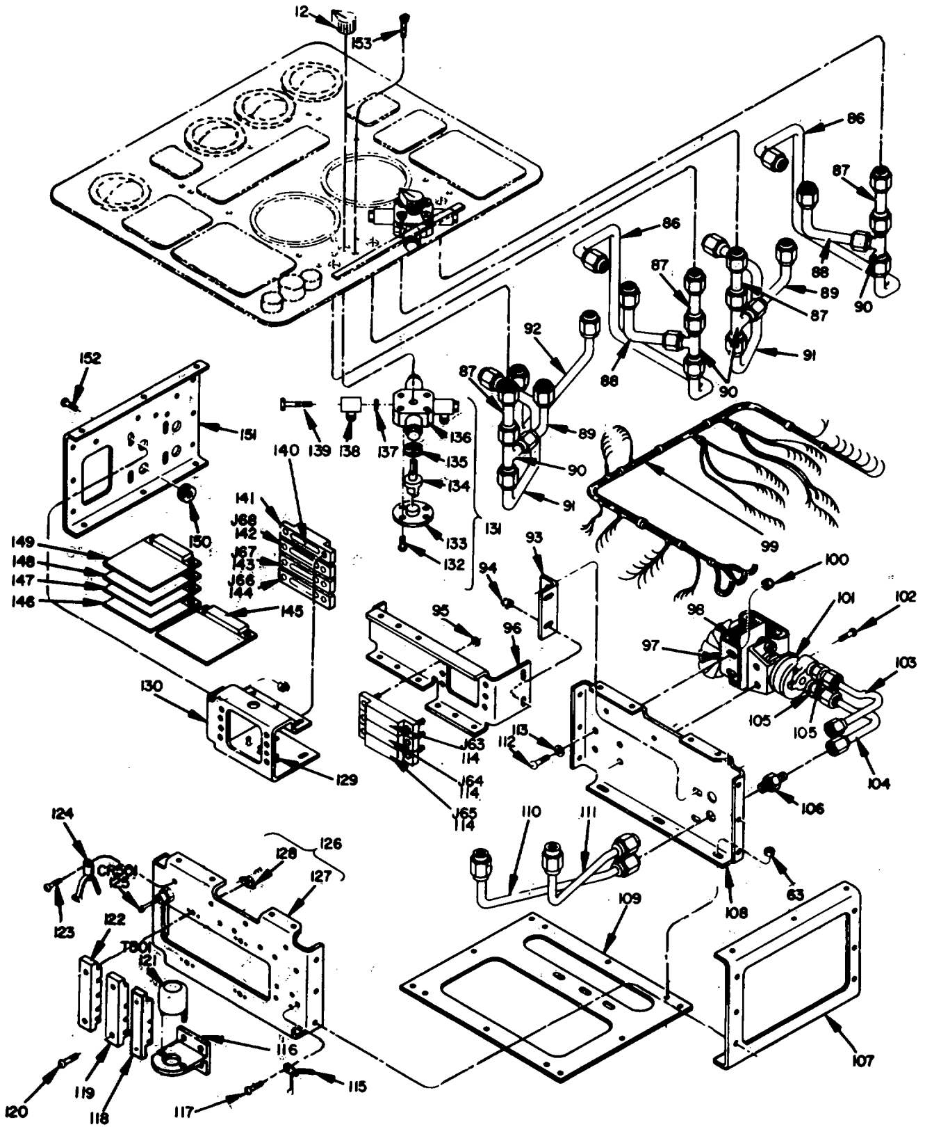
Figure 9. Panel Assembly, Front 114E5987-7 (Sheet 2 of 2).
