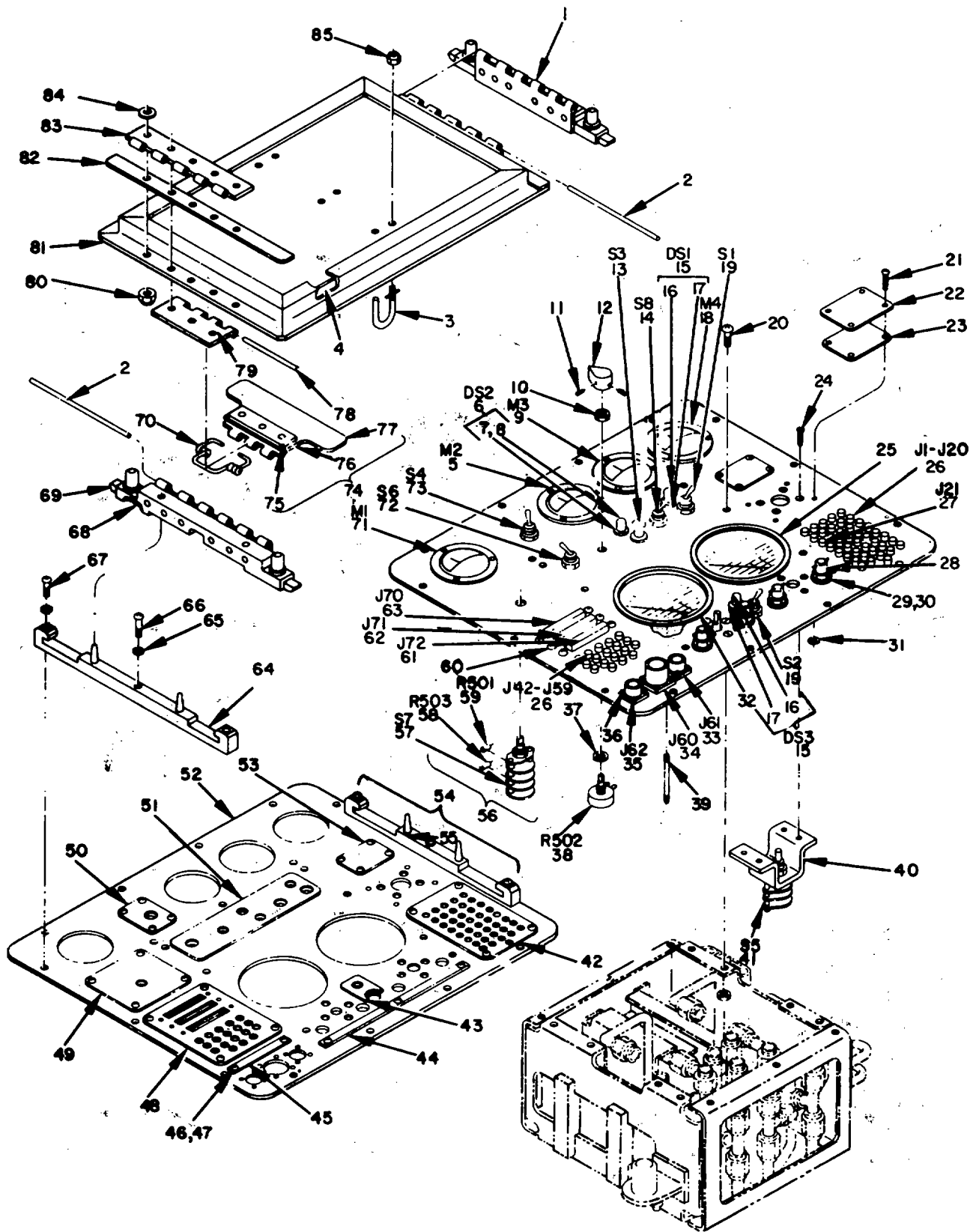
Figure 9. Panel Assembly, Front 114E5987-7 (Sheet 1 of 2).
