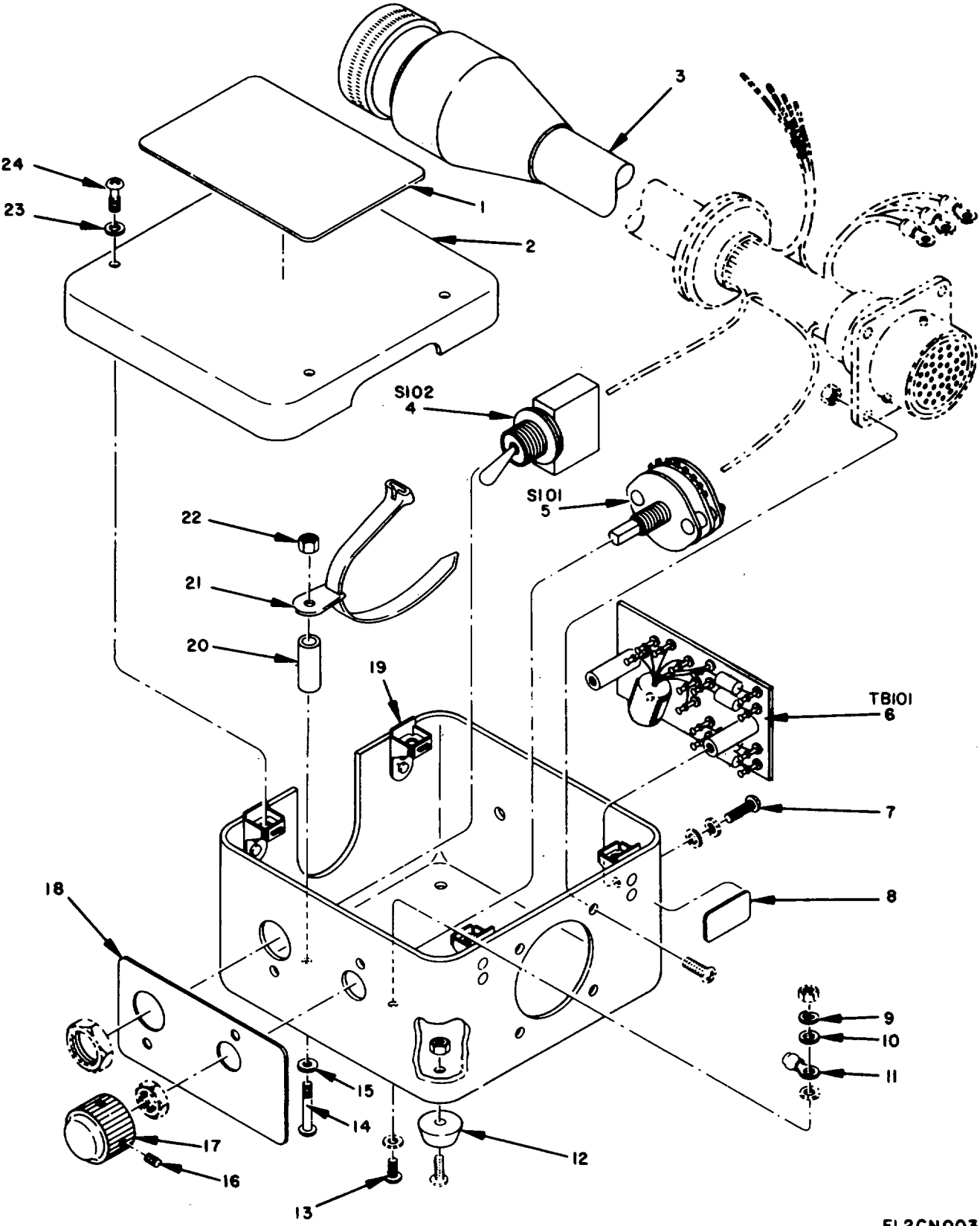
Figure 3. Box Assembly, Adapter 114V3058-1.
