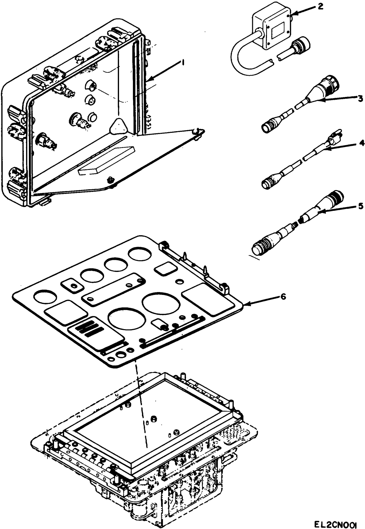
Figure 1. Test Set, Stabilization Equipment TS-1894/ASM.
