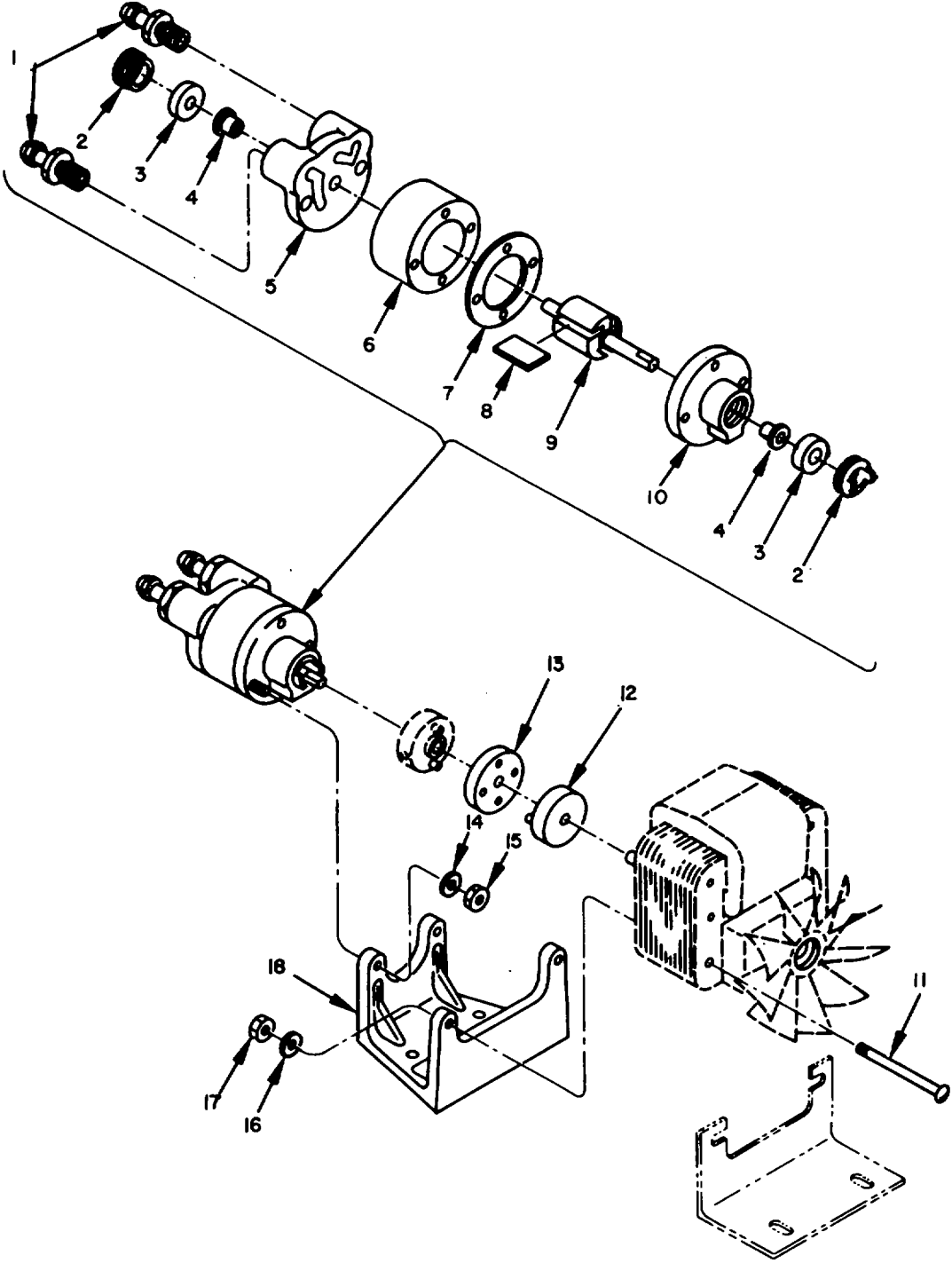
Figure 16. Pump Assembly, Air 0330P110-202.
