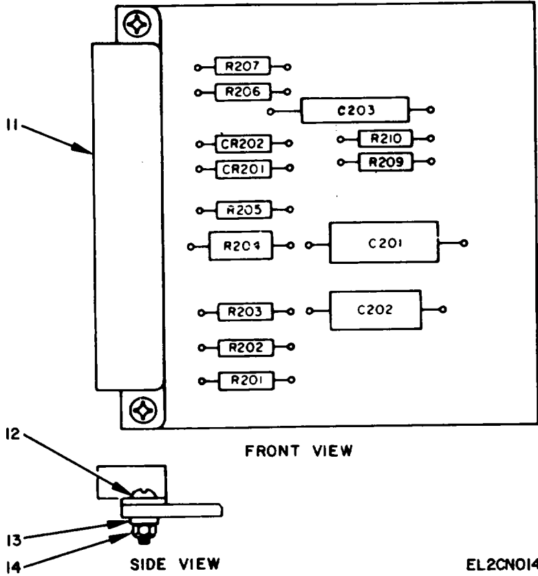
Figure 12. Component Assembly, Card A02V3060-2.
